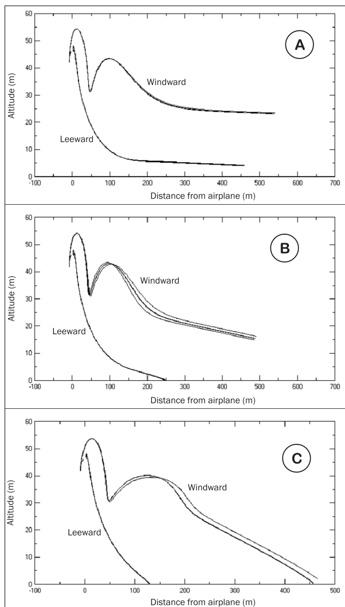
Figure 7. AGDISP model predicted trajectory of an (A) 22.3 \mu\text{m} droplet ( DV_{10} ), (B) 54.3 \mu\text{m} droplet ( DV_{50} ), and (C) 104.7 \mu\text{m} droplet ( DV_{90} ) from the C-130H airplane at 46 m release height. Windward and leeward annotations indicate the side of the airplane from which the droplets were released.
