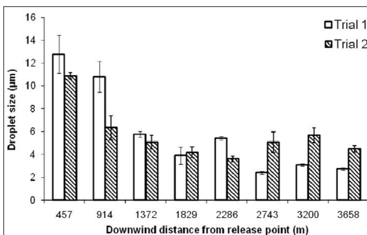
Figure 5. Average droplet size recovered from USAF C-130H fuselage mounted boom sprays using 8005 flat-fan nozzles at 91 m release height, February 17, 2005. (Bars are \pm 1 standard error.)
